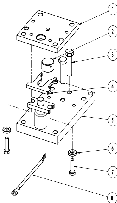
PROCEDURE FOR ASSEMBLING THE WEIGH MODULE
