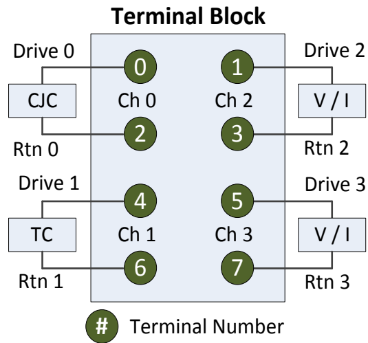
Figure 2-13. System Configuration 10 Thermocouple with Voltage or Current
