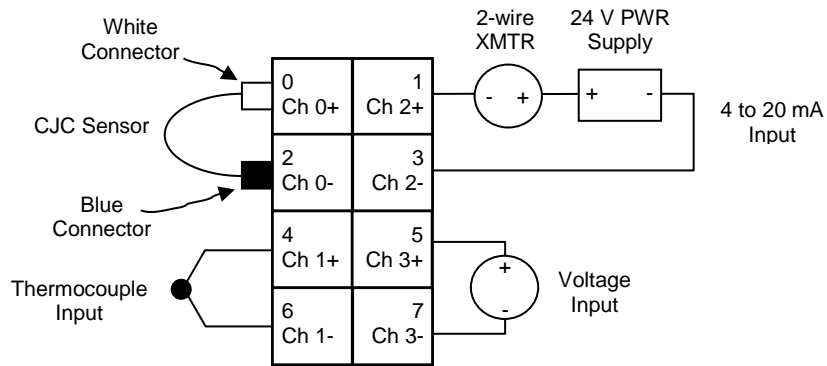
Figure 2-1. Voltage, Current, and Thermocouple
